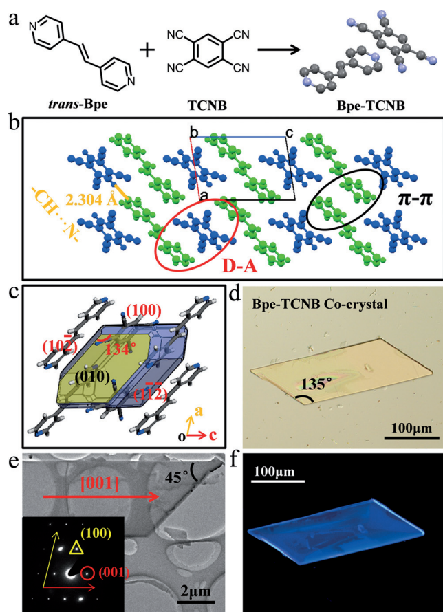
Figure 1. a) Chemical structure of trans -Bpe, TCNB, and the molecular structure of the resulting Bpe-TCNB complex. b) The self-assembly driving forces. c) The predicted equilibrium morphology of the cocystal. d) Optical image of BTC on the glass substrate. e) TEM and SAED images of individual BTCs. f) CLSM image of BTC on a glass substrate.
